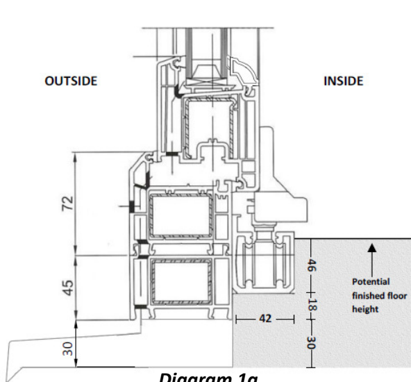
Diagram 1a Standard Threshold for Open IN doors
