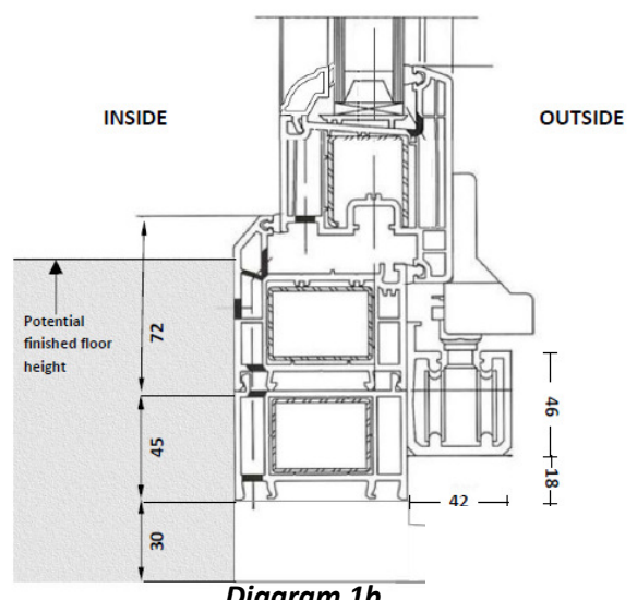
Diagram 1b Standard Threshold for Open OUT doors
